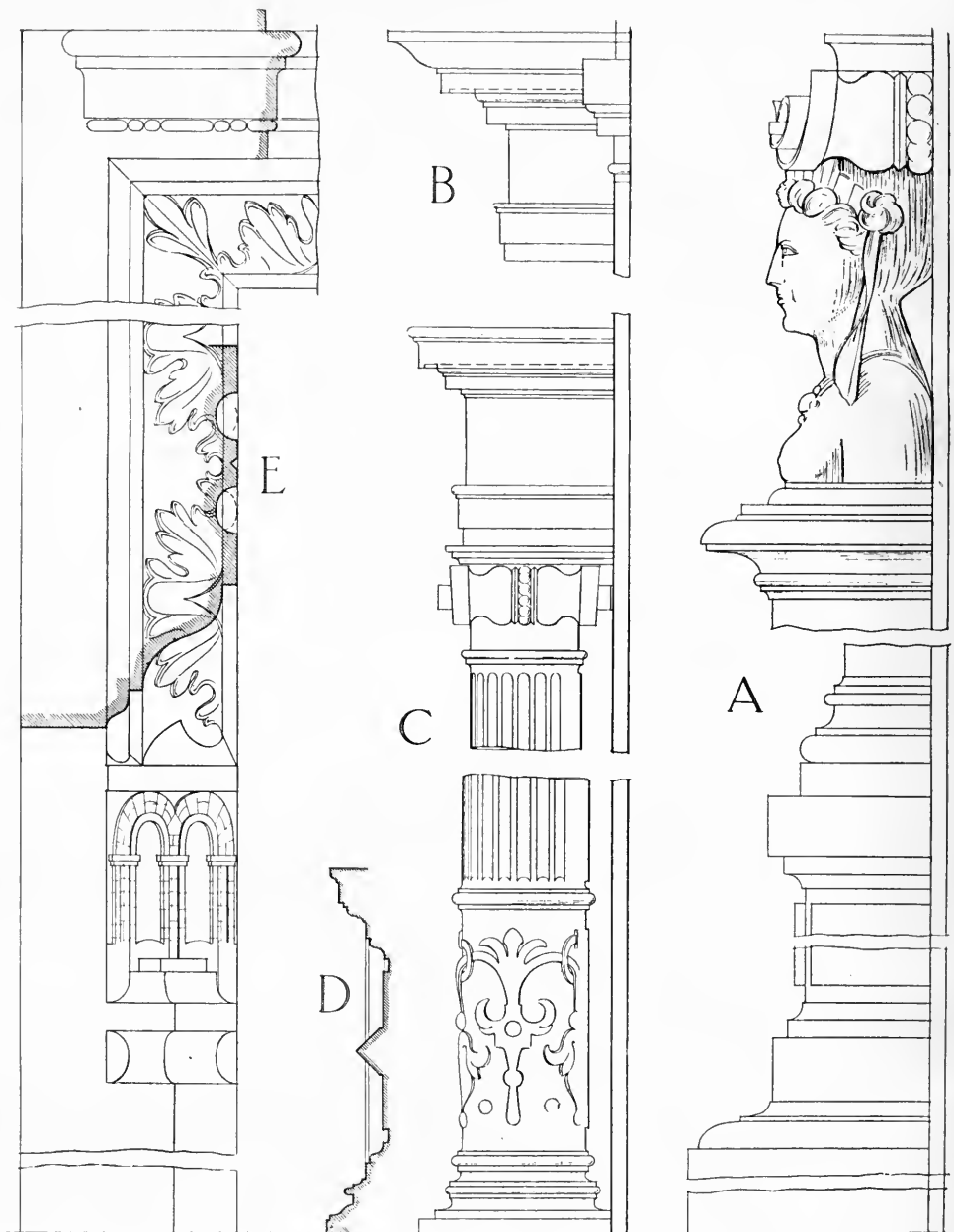
Measured drawing of sections of Chimney-piece.
